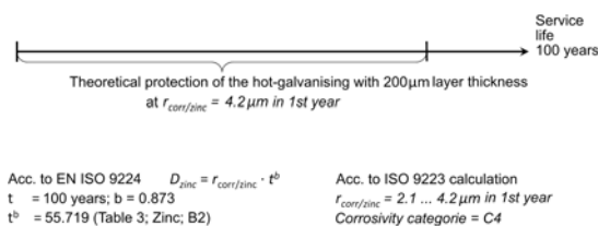
Fig. 4: Theoretical protection period for hot-dip galvanising (200 µm) [13]
