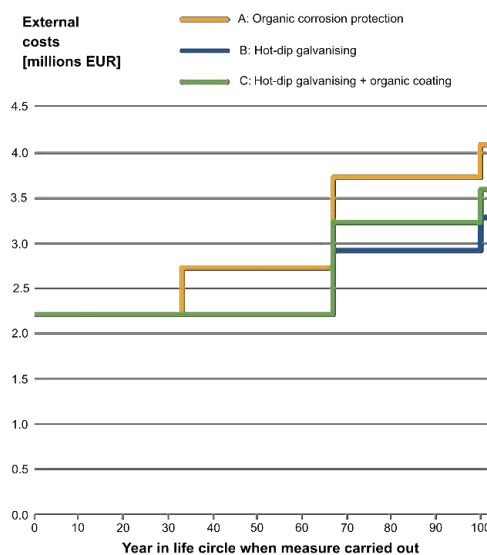
Fig. 28: External costs over the complete life cycle for the three variants [51]
